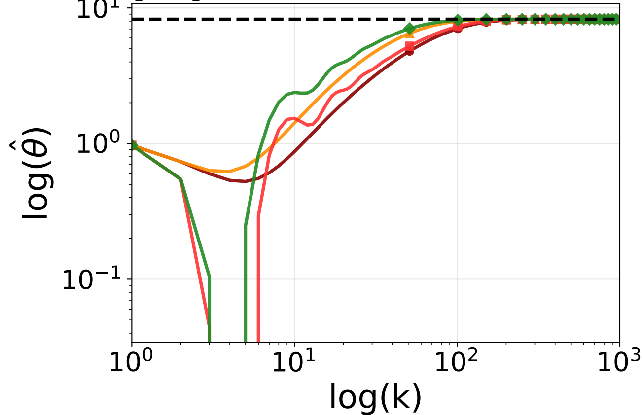
Log-Log Plot - D = 10, N = 20, X_0 \sim \mathcal{N}(0, 1)
